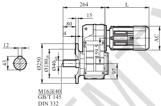
GFF67
