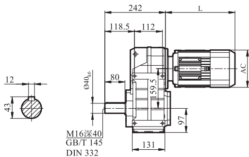
GFA/GFH/GFV67
